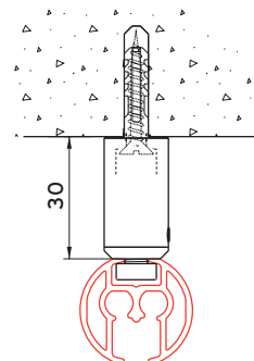
Ceiling fixing 5100 with mini-suspension hanger 4254
