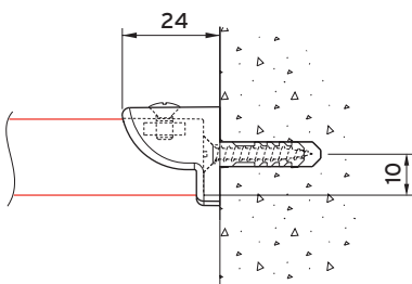
Wall fixing 4200 with wall support 4249
