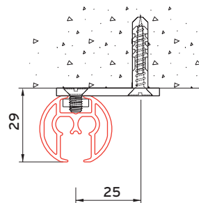
Ceiling fixing 5100 with bracket 5135
