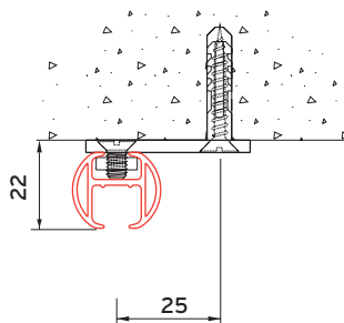
Ceiling fixing 4200 with bracket 5135
