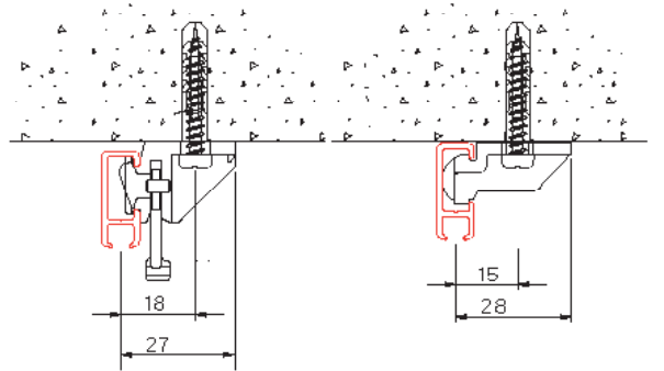
ceiling mounted with 7450 ceiling mounted with 2250
