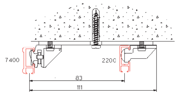
ceiling mounted with double bracket 2216 and 7450 or 2250
