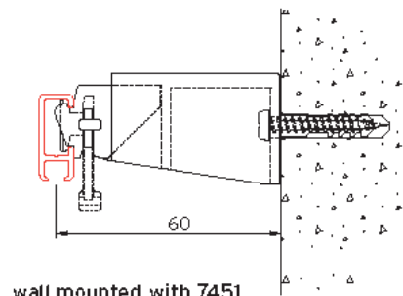
wall mounted with 7451
